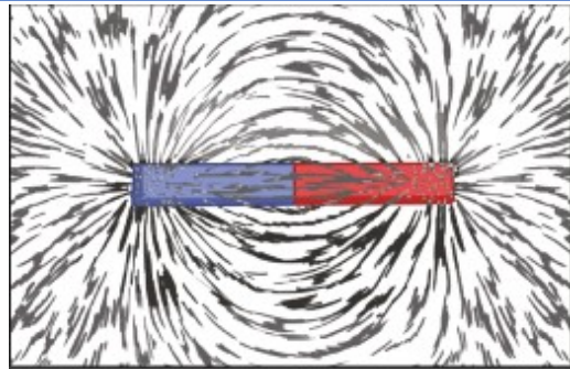
Magnetic Field
